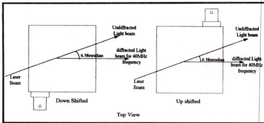
Fig. 1. AO device placed in the direction of laser beam.
