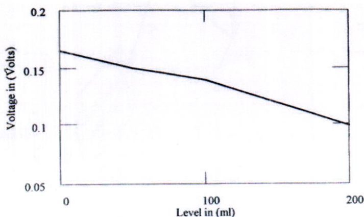
Fig 6. the peak output voltage from the linear detector versus the level of the liquid in ml.
