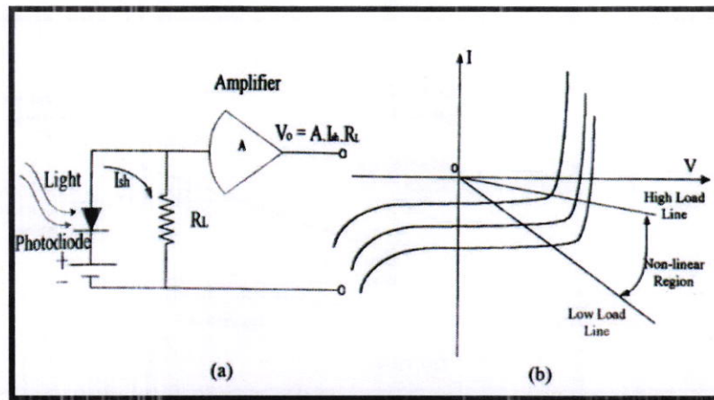
Fig.2. Nonlinear photodetector (a) Schematic diagram
