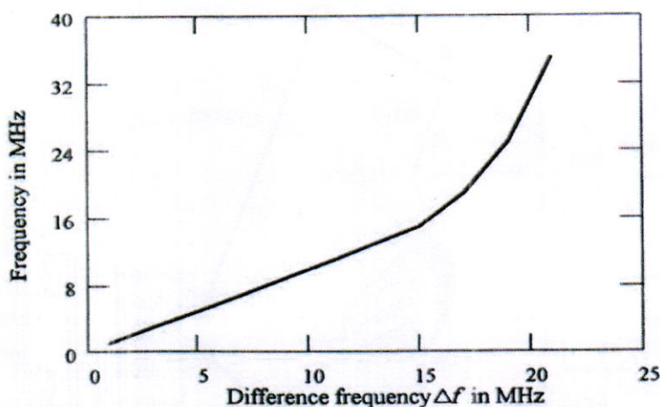
Fig.5 the response of the nonlinear detector for the two beam with difference in their frequency of \Delta f
