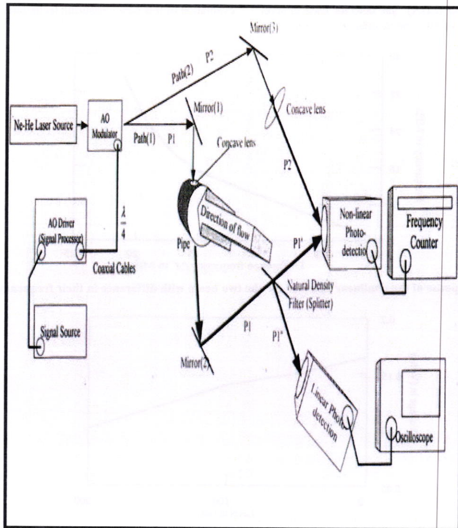
Fig 4. Schematic Diagram for system Measuring Flow rate and Level of a moving Liquid (oil).
