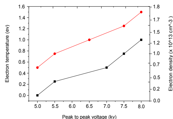
Figure 6: Electron density and electron temperature as a function of peak to peak applied voltage.
