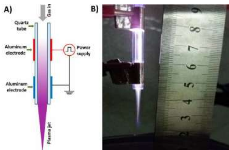
Figure 1: (A) Schematic diagram and (B) photograph of the DBD plasma jets .
