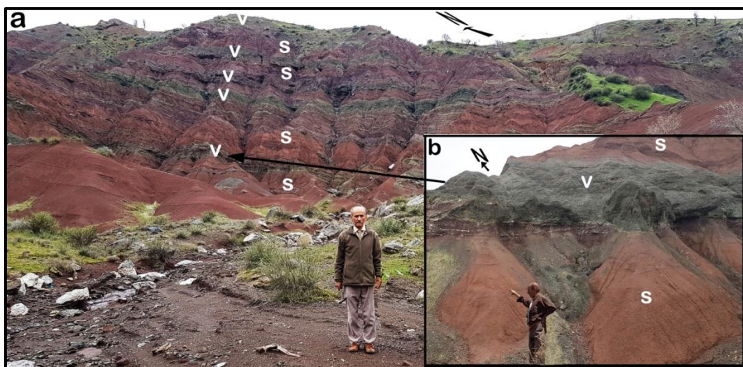
Fig.(22) Middle part of Red Bed Series at 2km west of Mawat town, contains several thick beds of volcaniclastic sandstone and conglomerate (V) interbedded with normal lithology (red claystone and sandstone) of the series (S),
