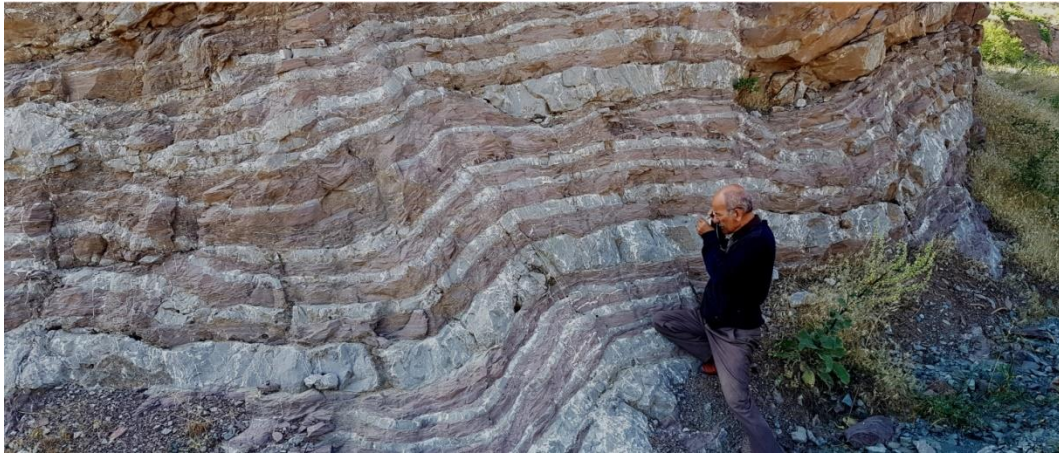
Fig. (10) Distal part of Naoperdan Formation as calciturbidite in western part of Mawat Metamorphic Core Complex (previous Mawat Ophiolite Complex) at 4 km northeast of Mawat town. The light layers consist of coarse detrital limestone which contains reworked nummulite forams. The dark layers are calcareous shale.
