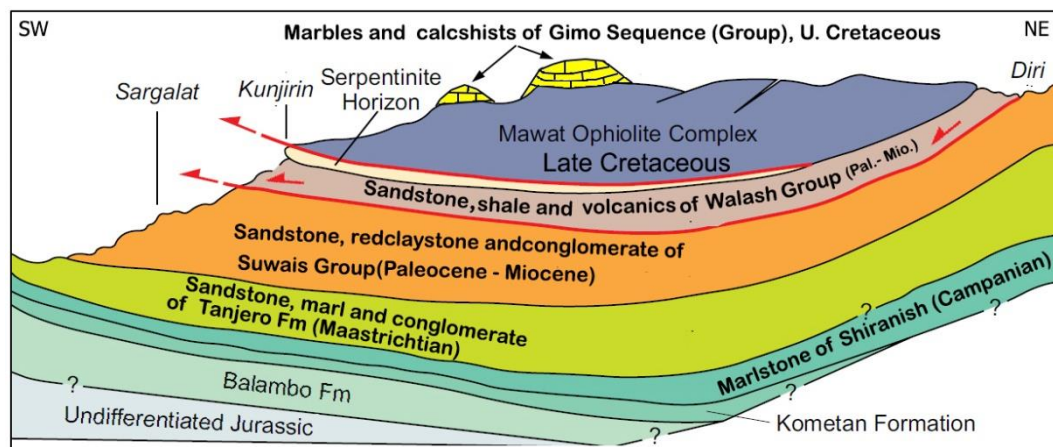
Fig. (5) Cross section of the Mawat Ophiolite Complex shows its tectonic stratigraphy and surrounding rock units (modified by Al-Qayim et al., 2012, from Mehaidi, 1975).
