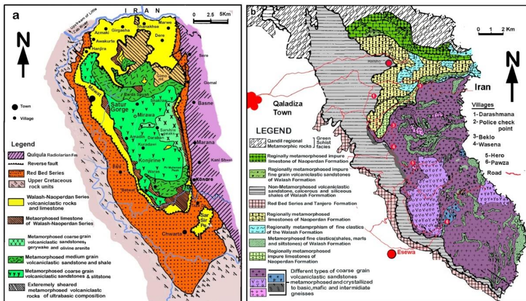
Fig.(27) Geological maps of Mawat (a) and Bulfat (b) on which the previous igneous rocks are replaced by metamorphosed sedimentary units.
