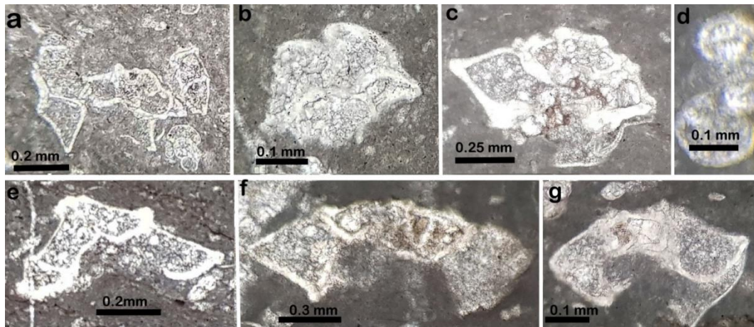
Fig. (18) Planktonic foraminifera inside the pelagic layers of Shiranish Formation in the Satur gorge belong to Upper Campanian, a) Globotruncana cf. ventricosa , b) Radotruncana subspinoso , c) Globotruncanita stuartiformis , d) Rugoglobigerina rugose , e) Contusotruncana, patelliformis , f) Globotruncana cf. insignis , g) Globotruncanita elevata
