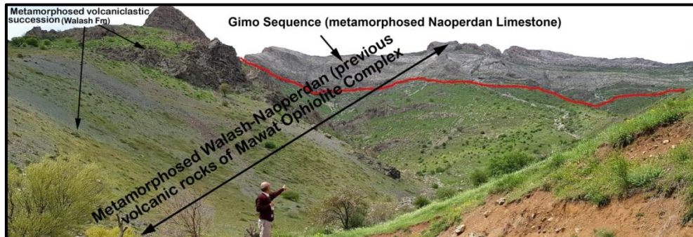
Fig.(11) A southern part of Gimo mountain show metamorphosed Naoperdan Formation (previous Gimo Sequence) and metamorphosed sandstone and siltstones of the Walash Formation (previous volcanic rock of Mawat Group), at the head of Saraw valley, south of Deri village
