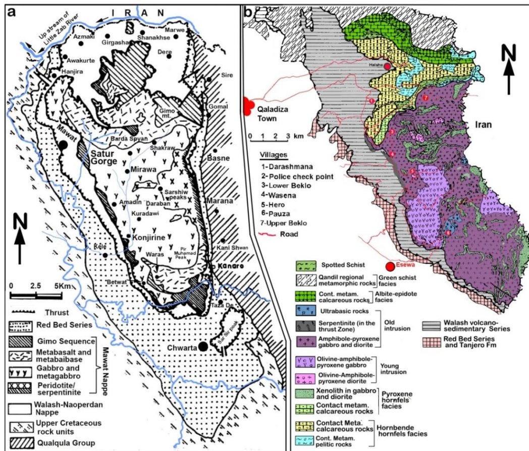
Fig.(2) a) Geological map of Mawat area (Al-Mehaidi,1975), b) Geological map of Bulfat (Qaladiza) area (Buda, 1993).
