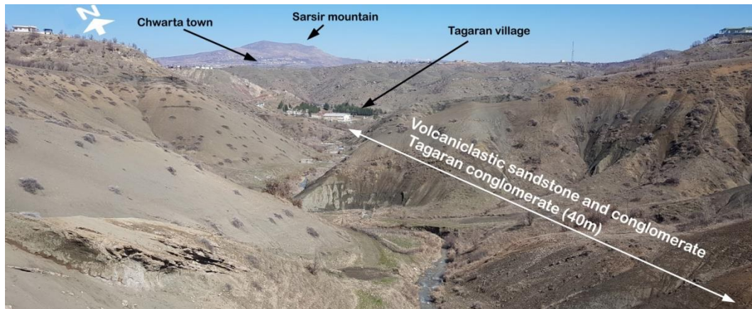
Fig. (20) Volcaniclastic sandstone (greywackes) and conglomerate at 1km south of Tagaran village at the base of Red Bed Series and t the top of Aqra Formation.
