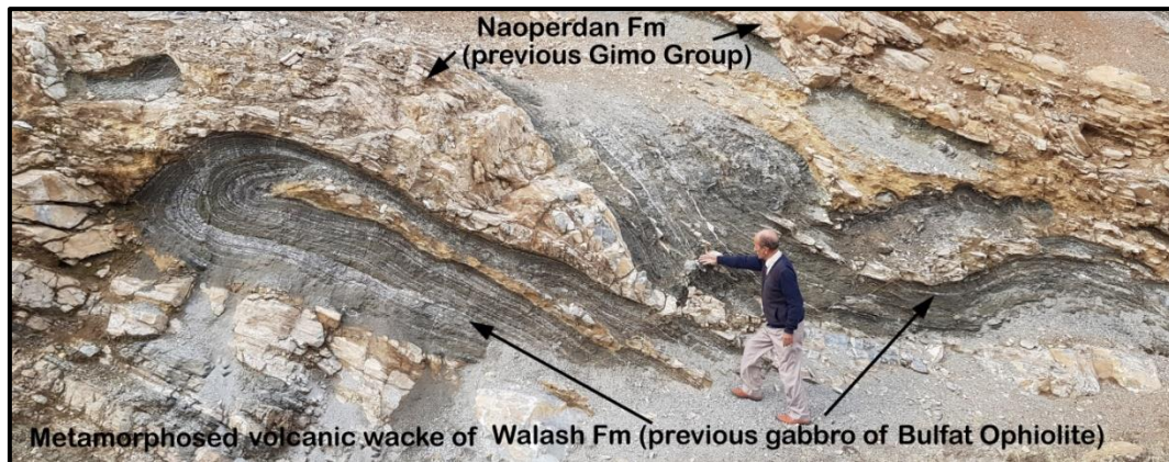
Fig.(13) Folded and laminated alternation of the greywacke (previous gabbro) and limestone of Naoperdan Formation (previous Gimo Sequence) which are regionally metamorphosed to green schist facies. The location is Bulfat Mountain at the middle of the paved road between Darashmana village and the Kele border police station. It can be seen that there are no contact metamorphism between the previous Gabbro and the limestone.
