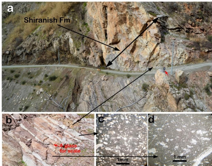
Fig.(16) a) general view of Satur gorge shows about 25 m of Shiranish Formation in the middle of the Walash Formations, the red arrow refers to a person for scale, b) close view of alternation of detrital and pelagic limestone beds forming calciturbidite, c) Thin section of detrital limestone under ppl, d) pelagic limestone contain planktonic foraminiferas.
