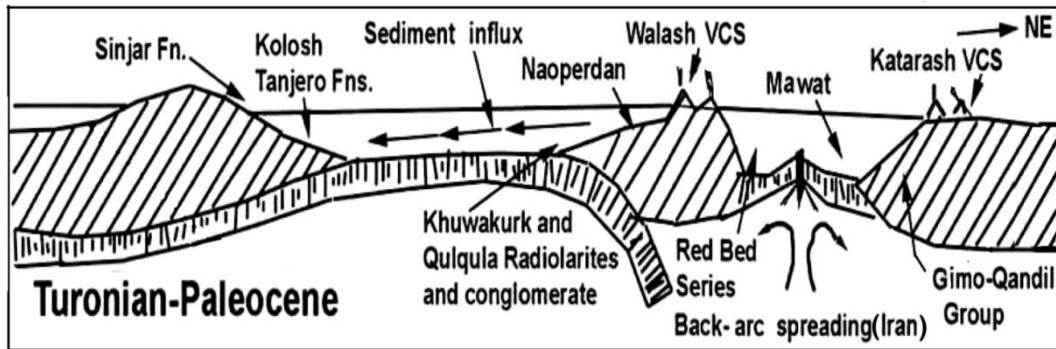
Fig. (25) Tectonic model of Zagros during Turonian-Paleocene (Numan, 1997), it can be very complex
