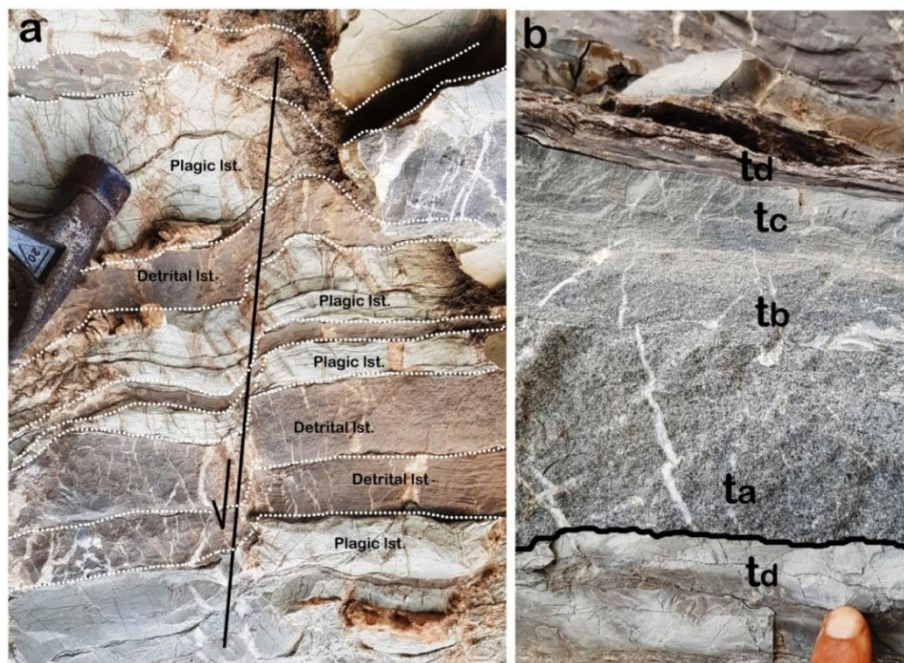
Fig. (17) a) alternation of detrital limestone (light brown) and pelagic limestone (white or light grey) of the Shiranish Formation in the Satur gorge. b) Detail of calciturbidite in the Satur Gorge shows division of the Bouma sequence.
