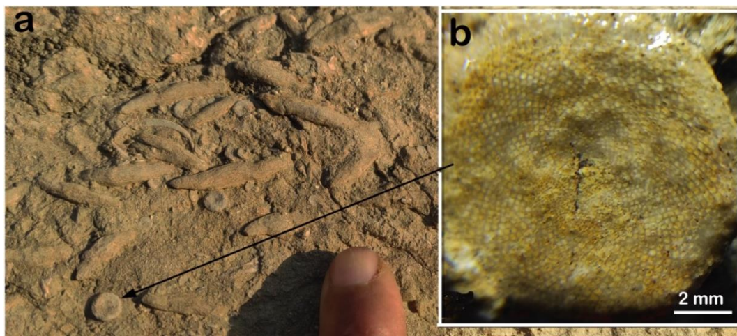
Fig. (21) Reworked Maastrichtian macrofossils in the lower part of the Red Bed Series in Chwarta area 500m southeast of Tagaran village, a) Loftusia, b) Amphalocyclus
