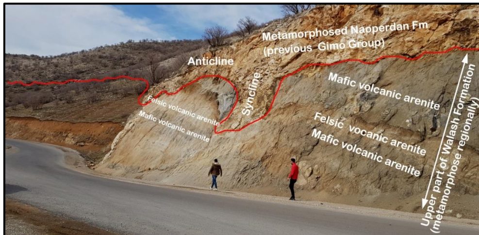
Fig.(12) the Bulfat Core Complex, like Mawat Metamorphic Core Complex, is capped (overlain) by metamorphosed limestone of the Naoperdan Formation (Previous Gimo Sequence) at 1km north of Biklo village on the paved road to Kele border Police station.
