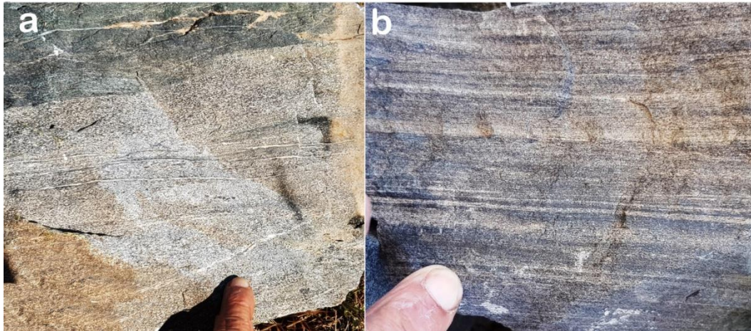
Fig.(6) Metamorphosed greywackes (previous gabbro and diorite of Mawat Complex) at 500 southwest of Syre village, a) lamination and cross bedding shaped by alternation of felsic and mafic laminae, b) planar lamination with felsic laminae (white) and mafic ones (black)
