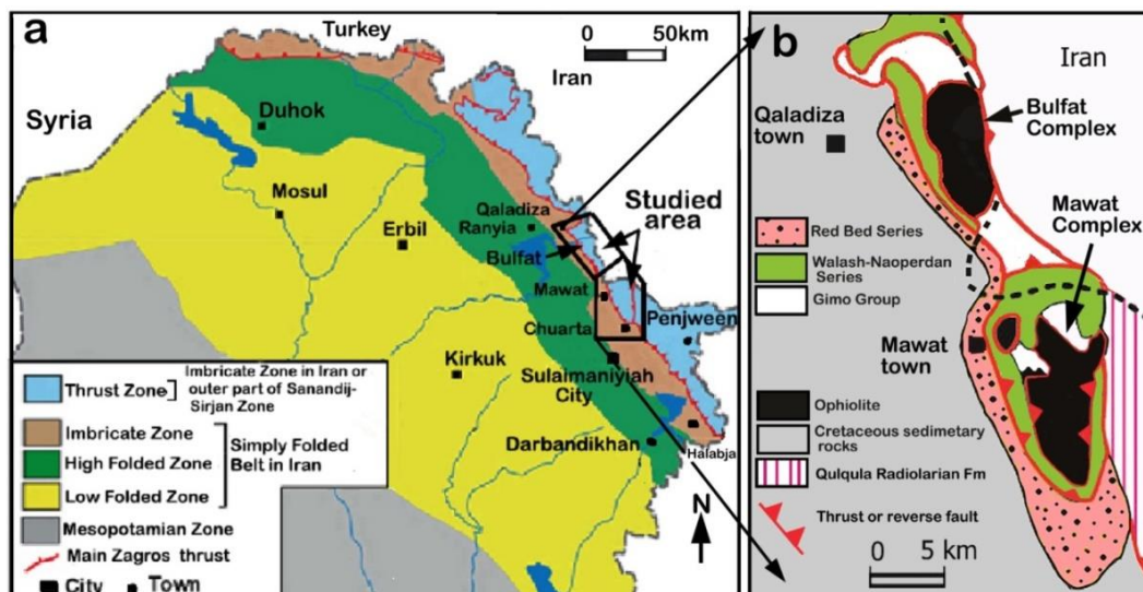
Fig. (1) a) Location map of the studied area on the tectonic map of northern Iraq (Jassim and Goff, 2006), b) Geological map of Mawat-Bulfat area (modified from Sisakian, 2000),
