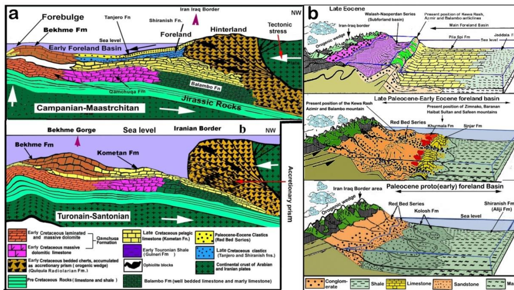
Fig.(28) a) Late Cretaceous tectonic models (Karim and Taha,2009) that agree with present study since there is not ophiolite obduction and opposes the models in the figures (Figs. 3 and 24). b) Realistic tectonic models (Karim et al. 2008) show how depocenter shifted toward northeast during Eocene.
