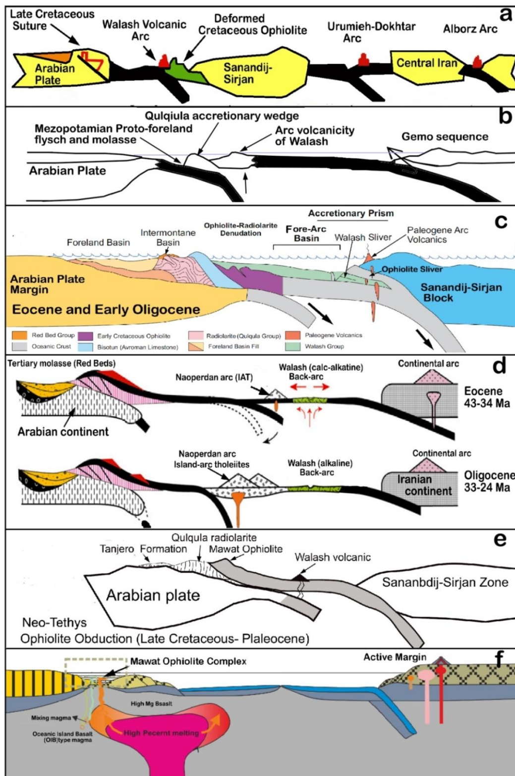
Fig.(3) Different tectonic models of previous studies show obduction of Mawat Ophiolite Complex and volcanism of Walsh Formation on an Island arc, a) Jassim and Goff (2006), b) Aziz et al (2011), c) Al-Qayim et al.(2012), d) Ali et al.(2013), e) Mohamad and Cornell, (2017), f) Azizi et al. (2013) this latter model shows development of Mawat area as an intrusion of mantle plume into an extensional tectonic regime on the thinned lithosphere of the Arabian passive margin.
