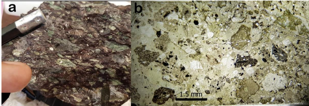
Fig. (7) a) volcaniclastic conglomerate at northeastern end of the Satur Gorge, 1km south of Gabarwa village, b) coarse volcaniclastic sandstone show volcanic clasts, 1km north Dashti Tile village at southwestern end on the latter gorge.
