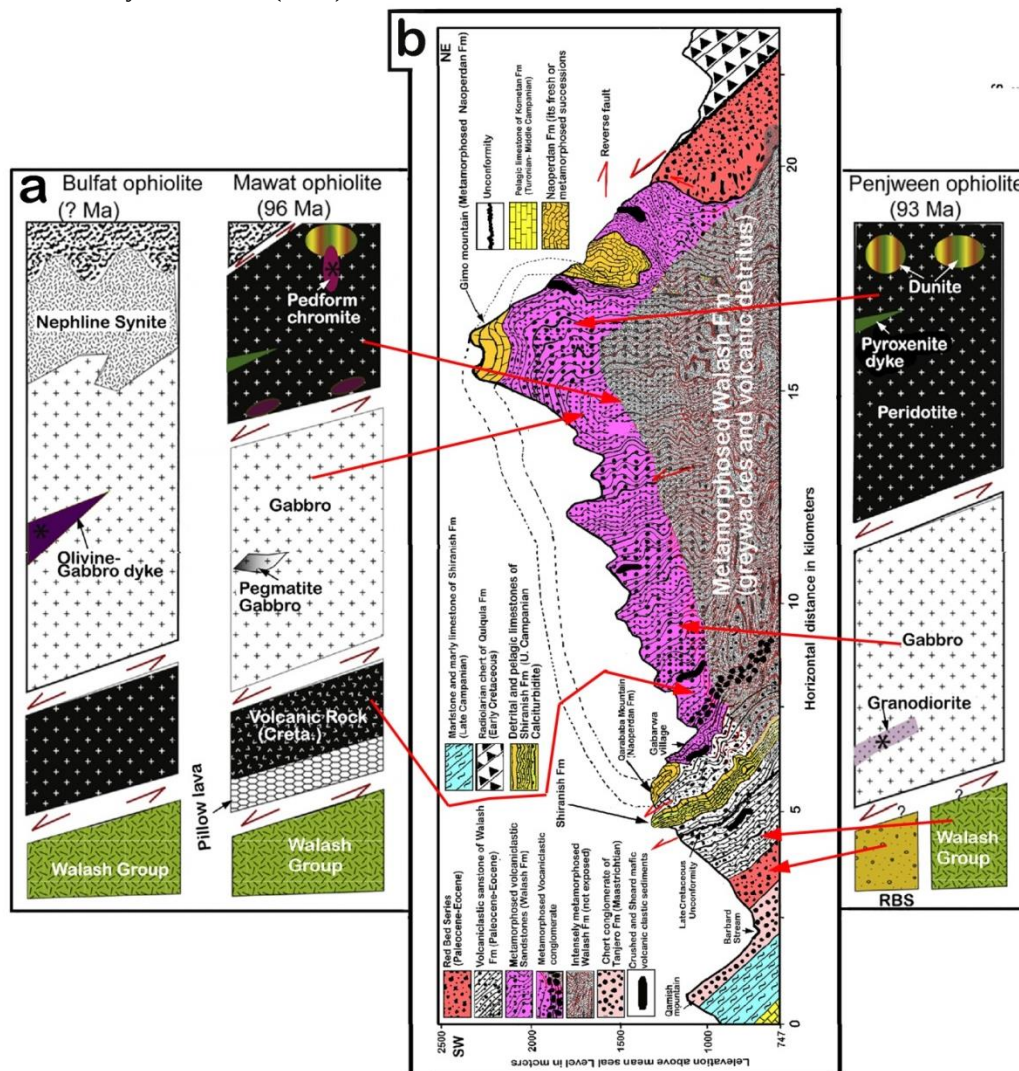
Fig. (24) a) Ophiolite section of the northeast Iraq by Ali et al. (2019) in which there are several thrusts sheet in the section of Mawat Bulfat and Penjween areas on which volcanic rocks and dunite located at the bottom and top of the sections respectively which oppose true section of ophiolite. b) True geologic cross section of the Mawat Metamorphic Core Complex shows true stratigraphic position of the two complexes (and Penjween area too which agree with age tectonic and fieldworks of the present study (the red arrows indicate correlated positions of the units of the present study with that Ali et al.(2019)
