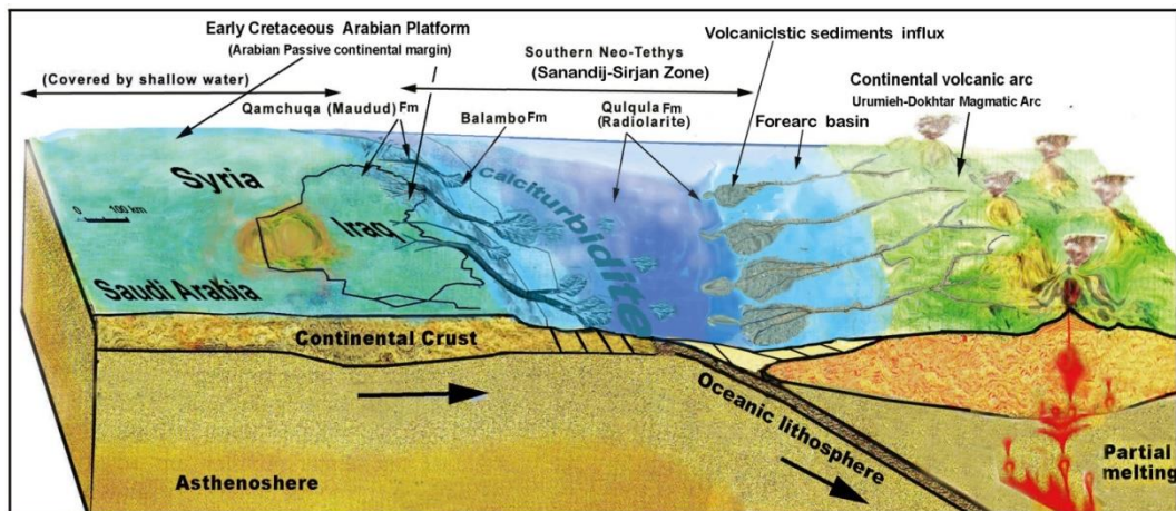
Fig.(26) Paleogeography and tectonic model of the Sanandij-Sirjan Zone (as part of the Neo-tethys sea) during Early Cretaceous (modified slightly from Karim, 2020).
