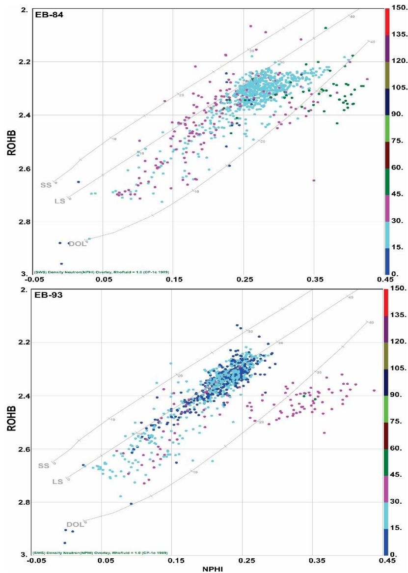
Figure 3. Neutron–density (NPHI–RHOB) plots of wells EB–84 (top) and EB–93 (bottom). Sandstone (SS), limestone (LS), and dolomite (DOL) lithology reference lines are indicated, together with porosity trends (10–40%). Most of the data lie on the limestone and dolomite trends, which means that the lithologies are carbonate with variable porosity. The limestone lines represent clean carbonate formations.
