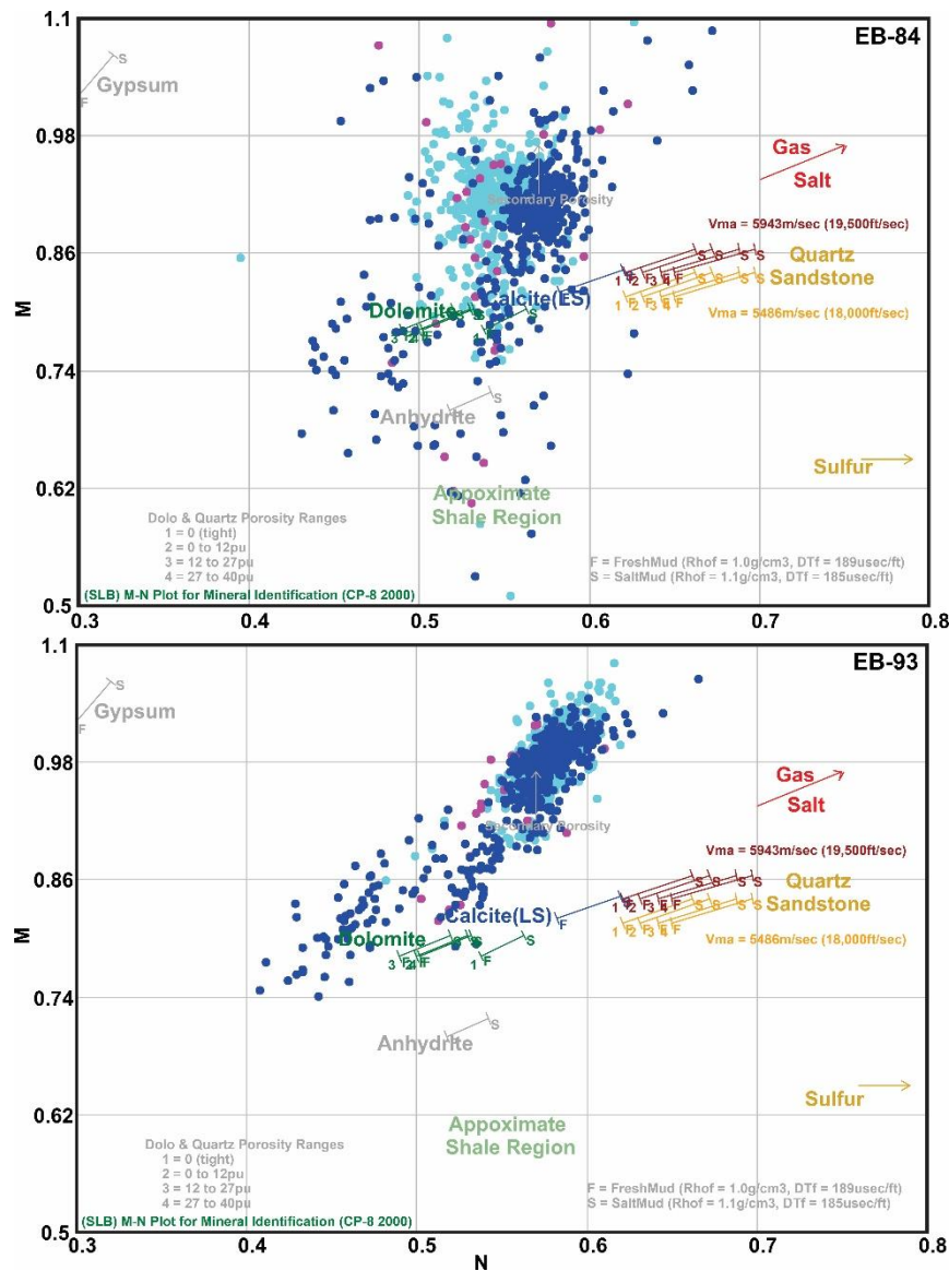
Figure 4. M–N plot of Well EB–84 (top) and Well EB–93 (bottom) to identify minerals and estimate porosity. Data points are clustering mostly on the trends of calcite (limestone) and dolomite, which validates the lithology of the Tanuma, Khasib, and Kifl formations, which are dominated by carbonates. The presence of clustering around the calcite line means that limestone is the dominant mineral, and the dispersion around the dolomite line means mixed dolomite intervals. The secondary porosity can be traced in the upward movement of the points, with minor scattering towards the shale area, indicating the localized influence of the clay. The separation of the plots with the quartz/feldspar trends also supports the characterization of the carbonate reservoirs.
