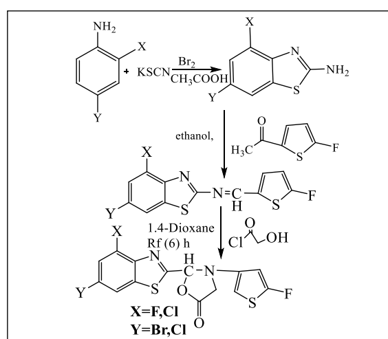
Fig. 3. Route of prepared compounds (W1-9)
