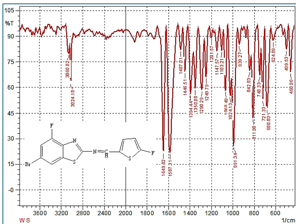
Fig. 7. The compound's FT-IR spectra(W 4 )
