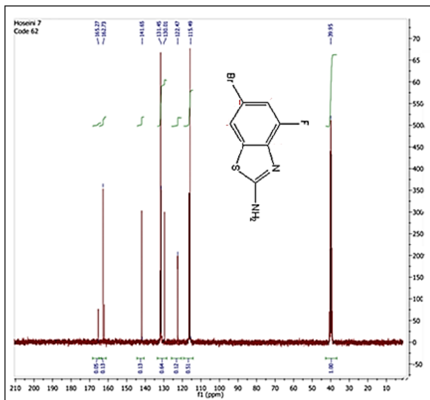
Fig. 6. CNMR spectra of the substance(W 1 )
