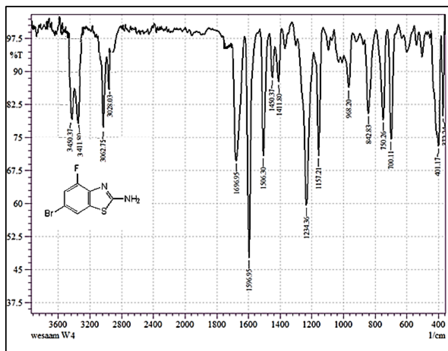
Fig.4. the compound's FT-IR spectra(J1) (W 1 )
