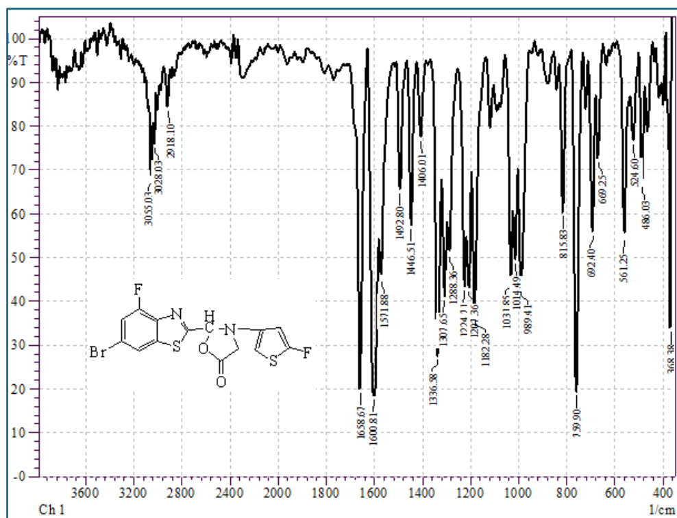
Fig. 10. The compound's FT-IR spectra(W7)
