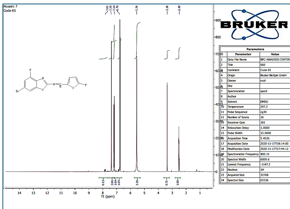
Fig. 8. 1-H NMR spectra of the substance(W 4 )
