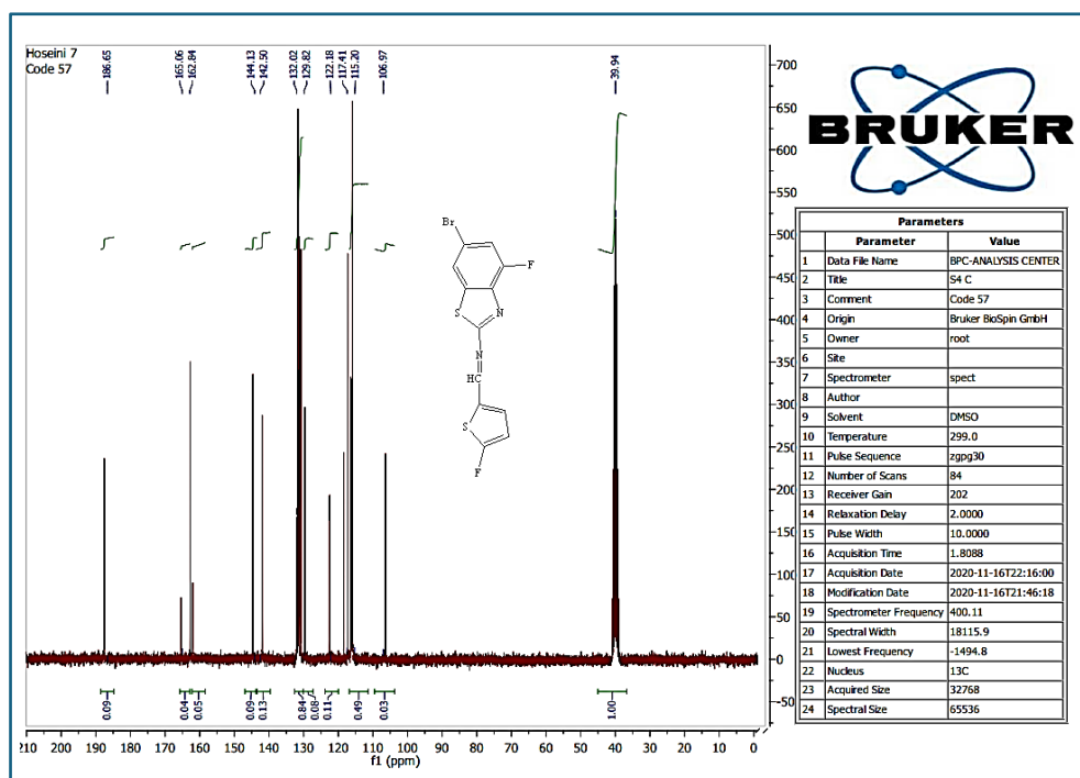
Fig. 9. CNMR spectra of the substance(W 4 )
