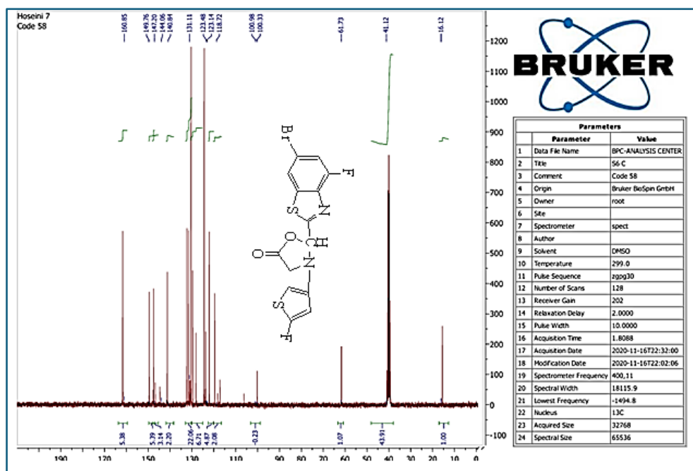
Fig. 12. CNMR spectra of the substance(W 7 )
