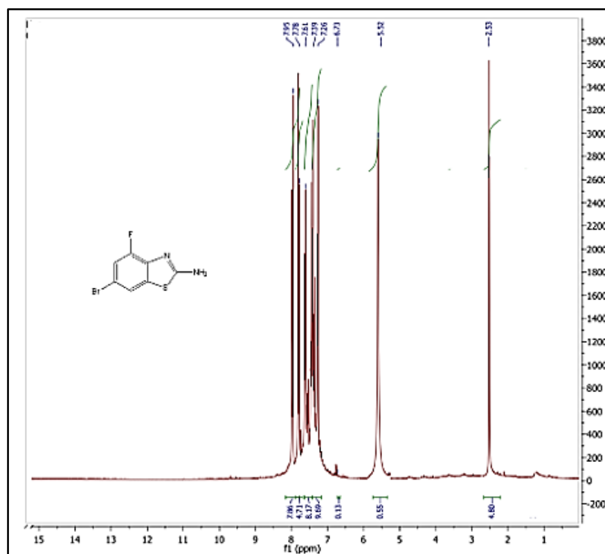
Fig. 5. 1-H NMR spectra of the substance(W 1 )
